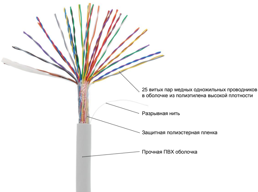
NTX-UU025-5-PVC-GY-3
