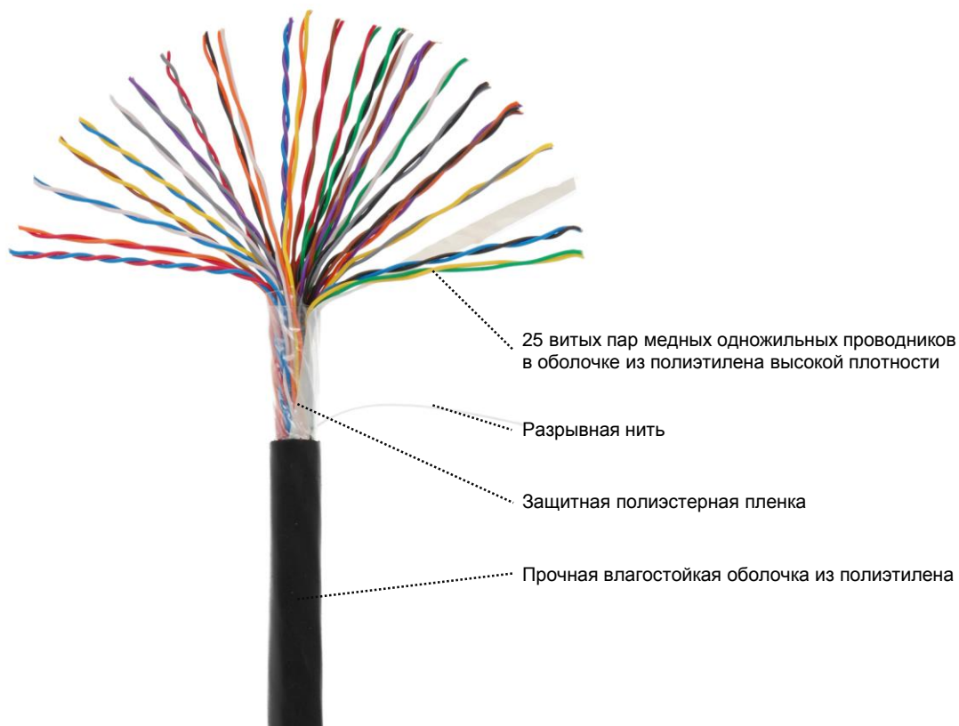
NTX-UU025-5-PE-BK-3
